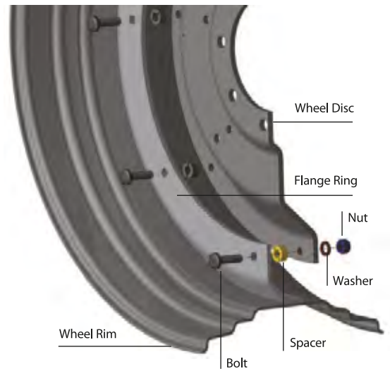
Partial exploded view of a typical MAVT wheel
